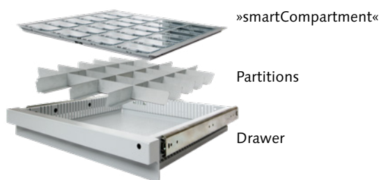
Drawer components
